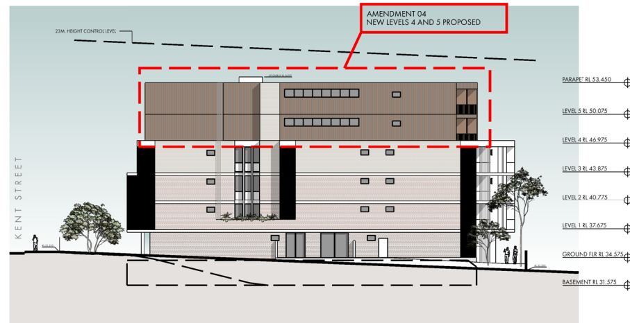
SOUTH ELEVATION
