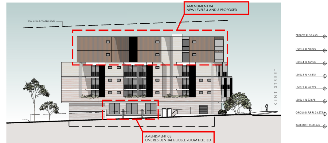
NORTH ELEVATION
